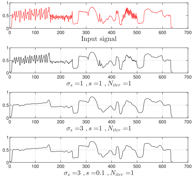
FIGURE 4: Filtering a 1D signal using the proposed GVWA filter with different parameter settings and no iteration.
