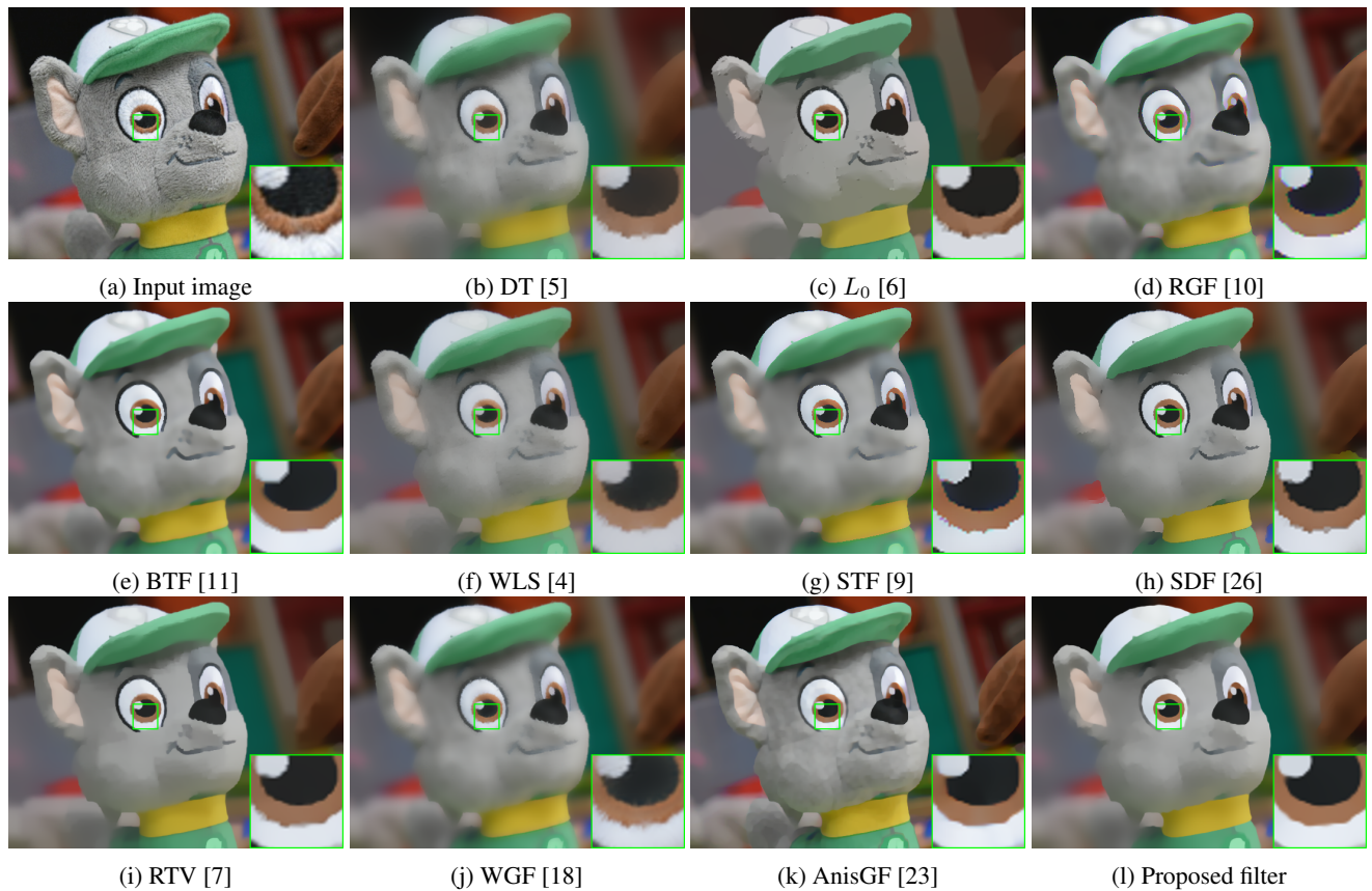
FIGURE 7: A comparison of edge-preserving image smoothing with a group of state-of-the-art algorithms. (a) Original image, (b) DT ( \sigma_s = 30, \sigma_r = 0.7, N_{iter} = 5 ), (c) L_0 ( \lambda = 0.02, \kappa = 2, N_{iter} = 1 ), (d) RGF ( \sigma_s = 5, \sigma_r = 0.1, N_{iter} = 20 ), (e) BTF ( k = 5, N_{iter} = 5 ), (f) WLS, ( \lambda = 1, \alpha = 1.2 ), (g) STF ( \sigma_s = 3, \sigma_r = 0.08, \sigma = 0.01, N_{iter} = 4 ), (h) SDF ( \sigma_g = 50, \sigma_u = 400, \lambda = 30, nei = 1 ), (i) RTV ( \sigma = 3, \lambda = 0.015, \epsilon = 0.02, N_{iter} = 4 ), (j) WGF ( \sigma = 1, \epsilon = 0.01, N_{iter} = 10 ), (k) AnisGF ( \sigma = 1.5, \epsilon = 1 ) (l) Proposed rolling GVWA Type-II filter ( \sigma_s = 1.5, s = 0.75, N_{iter} = 20 ).
